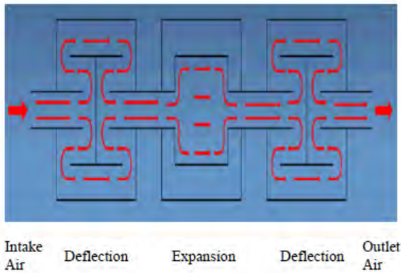
Figure 4: Flame arrester schematic drawing
